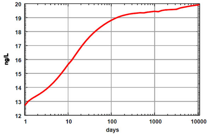
Figure 7. The concentration of uranium in the urine of adults with continual ingestion of 1 \mu\text{g/L} .
