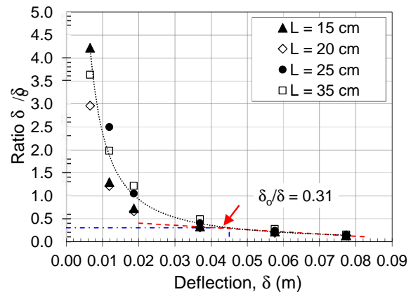
Figure 5: The relationship between the deflection of slabs ( u ) and the ratio of u/u_0
