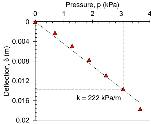
Figure 6: The Modulus of subgrade reaction values
