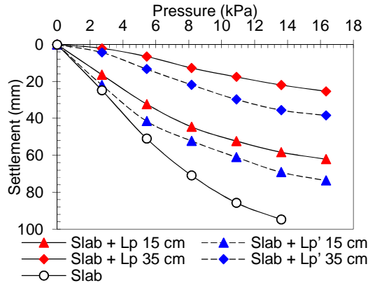
Figure 9: The relationship between pressure due to embankment and settlement at the center of embankment
