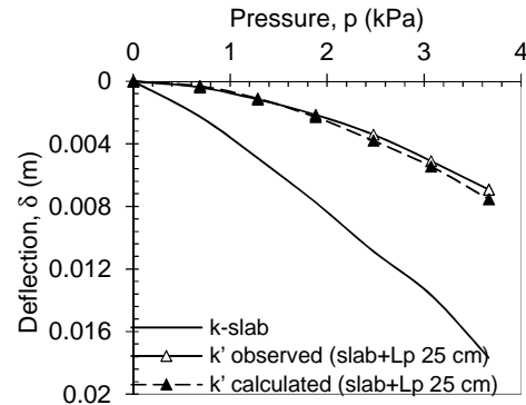
Figure 7: The comparison between calculated and observed deflection
