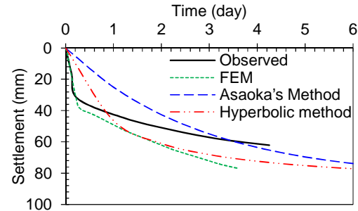
Figure 13: The relationship between time and settlement of slabs with piles
