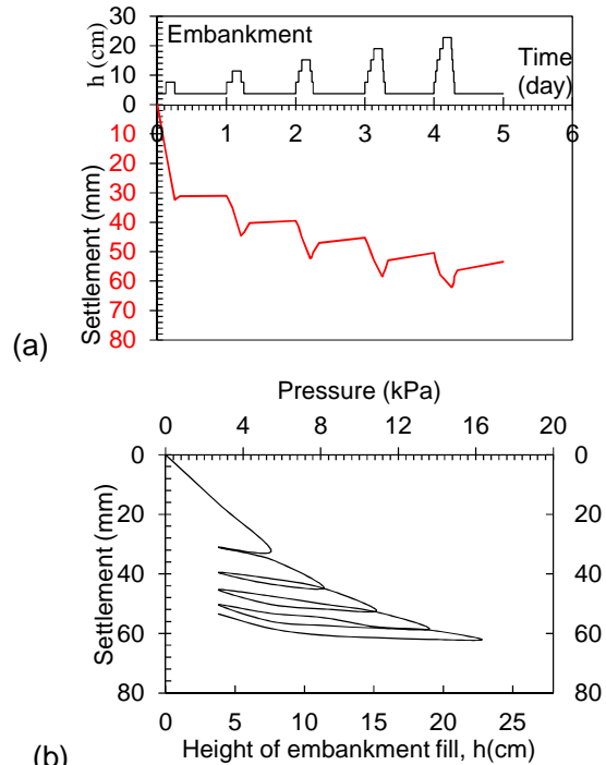
Figure 8: The settlement in the center of embankment on slabs with 15 cm monolithic piles: (a) The relationship of time and settlement; (b) The relationship between pressure and settlement
