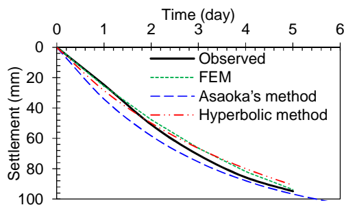
Figure 12: The relationship between time and settlement of slabs without piles
